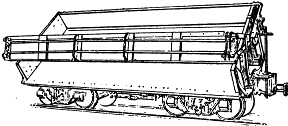
Fig. 111. An 8-Yd. Car in Dumped Position.
